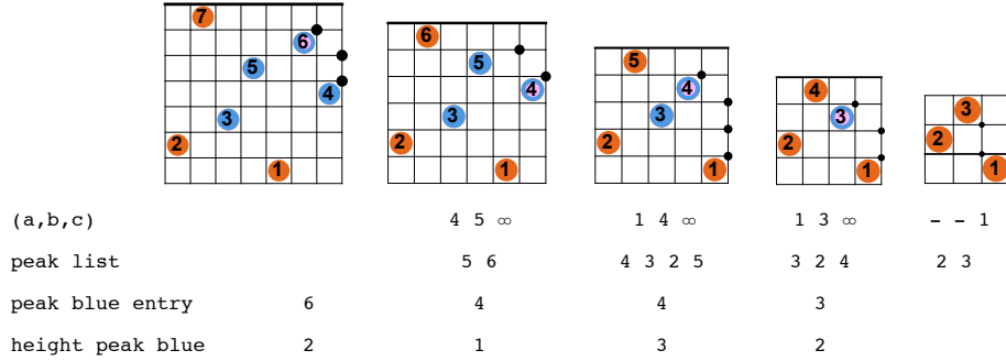
Fig. 4: An example of the bijection.
