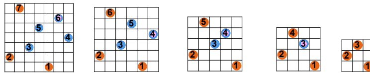
Fig. 2: Avoiders with colored entries and highlight.
