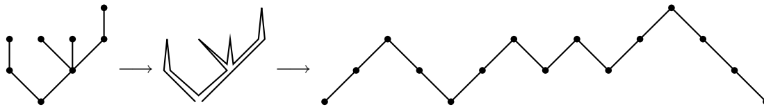
The “accordion” bijection
