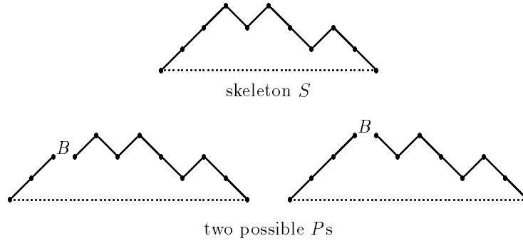
Recapturing a path P \in \mathcal{P}[DUU] from a skeleton S and body B
