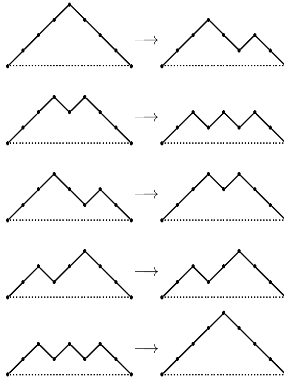
action of F on primitive Dyck 4-paths
