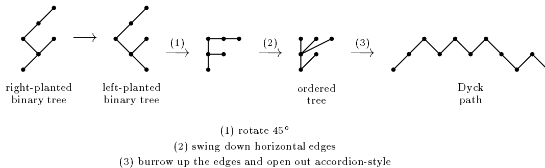
binary tree \leftrightarrow Dyck path correspondence
