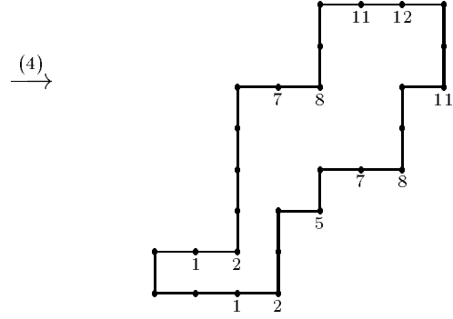
(4) subtracts 1 from each label in upper path, and to restore the counting of steps from (0,1) in the upper path and from (1,0) in the lower path amounts to rotating the initial (vertical) step in each path 90° counterclockwise
