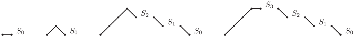
decompositions of nonempty Schröder paths
