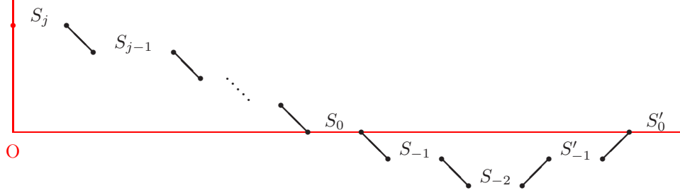
decomposition of path in \mathcal{A}_{j,d}
