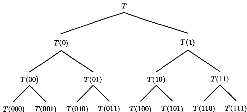
FIGURE 8.5.1 Computation Tree
