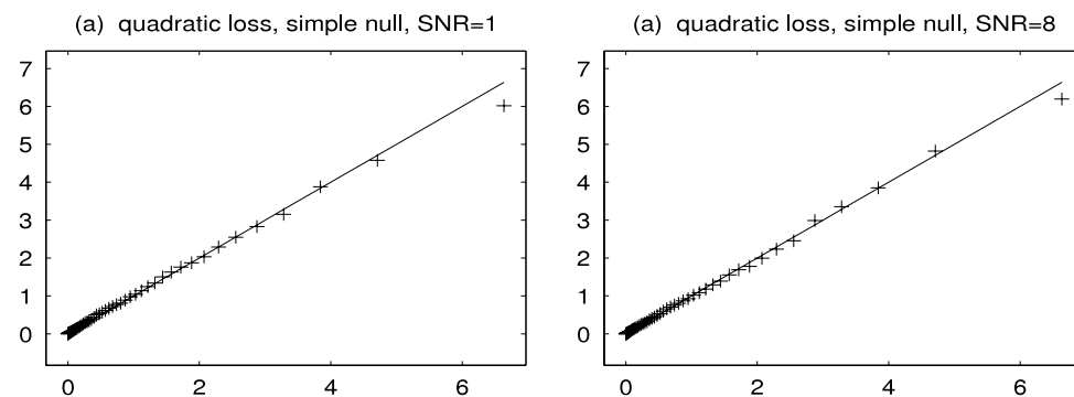
Fig. 3. (Simulated fMRI series in one voxel.) Empirical quantiles (on the y-axis) of test statistics W_n versus quantiles (on the x-axis) of the \chi_1^2 distribution. Solid line: the 45° reference line. The null hypothesis is H_0 : h(t_9) = 0 .
