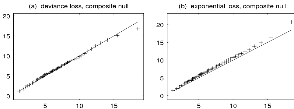
Fig. 10. (Simulated Bernoulli responses.) Empirical quantiles (on the y-axis) of test statistics W_n versus quantiles (on the x-axis) of the \chi^2_7 distribution. Solid line: the 45° reference line. The null hypothesis (6.4) is considered.
