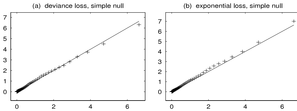
Fig. 9. (Simulated Bernoulli responses.) Empirical quantiles (on the y-axis) of test statistics W_n versus quantiles (on the x-axis) of the \chi^2_1 distribution. Solid line: the 45° reference line. The null hypothesis (6.3) is considered.
