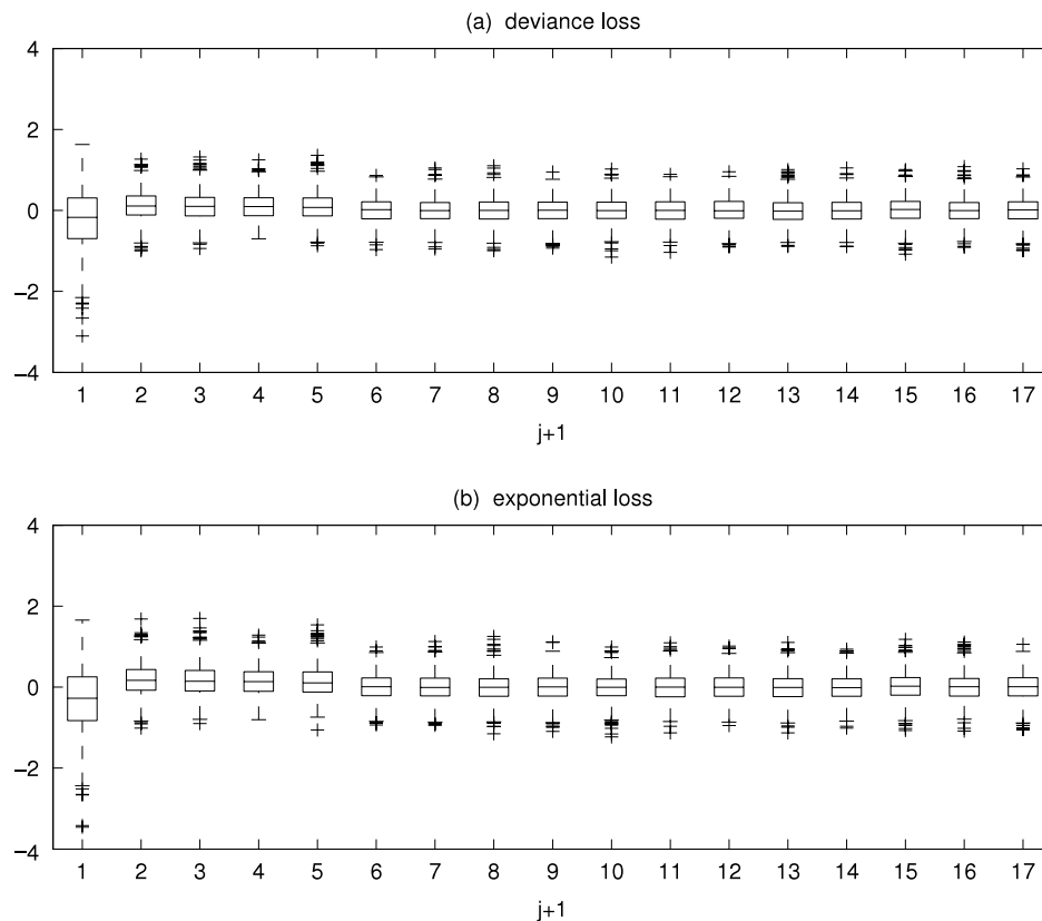
Fig. 8. (Simulated Bernoulli responses.) Boxplots of \hat{\beta}_{n,j} - \beta_{n,j;0}, j = 0, 1, \dots, p_n (from left to right in each panel). Panel (a): using the deviance loss; panel (b): using the exponential loss.
