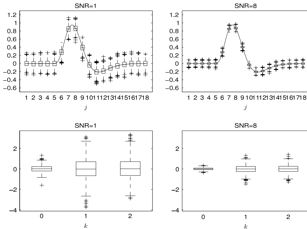
Fig. 2. (Simulated fMRI series in one voxel.) Top panel: boxplots of \widehat{h}(t_j), j = 1, \dots, p_n , where the solid line denotes the true h(\cdot) . Bottom panel: boxplots of \widehat{\alpha}_k - \alpha_k, k = 0, 1, 2 .
