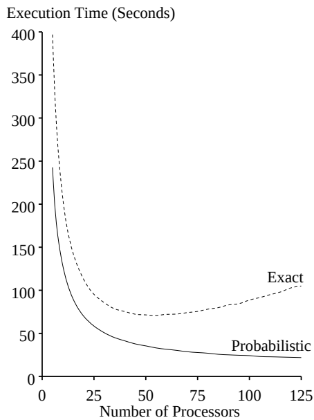
Figure 1: Analytic model predictions for sorting 1M tuples.
