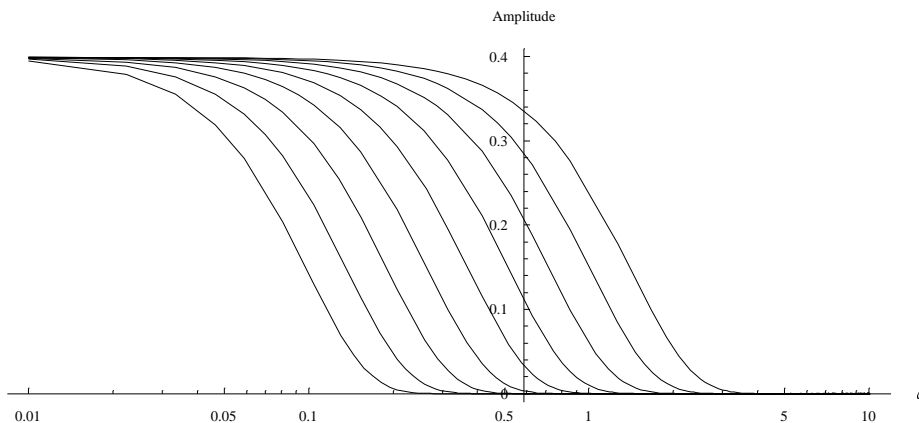
Figure 3.14. Fourier spectra of the Gaussian kernel for an exponential range of scales \sigma = 1 (most right graph) to \sigma = 14.39 (most left graph). The frequency \omega is on a logarithmic scale. The Gaussian kernels are seen to act as low-pass filters.
