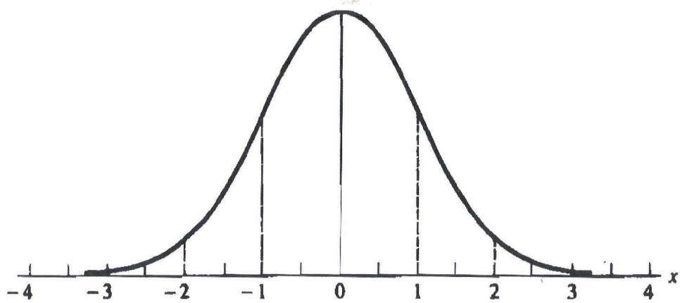
Figure 3.3.1. Standard normal density
