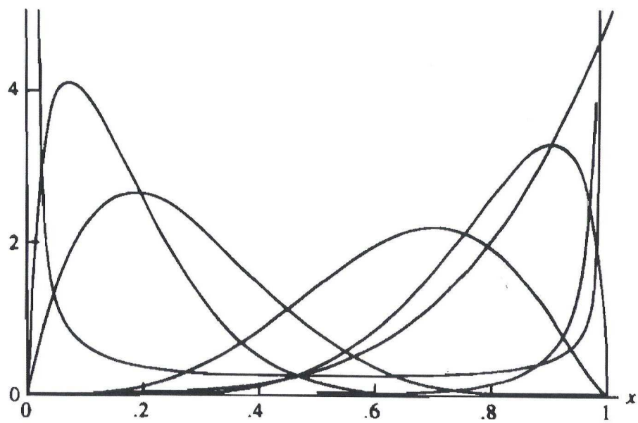
Figure 3.3.3. Beta densities
