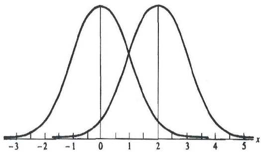
Figure 3.5.1. Two members of the same location family: means at 0 and 2
