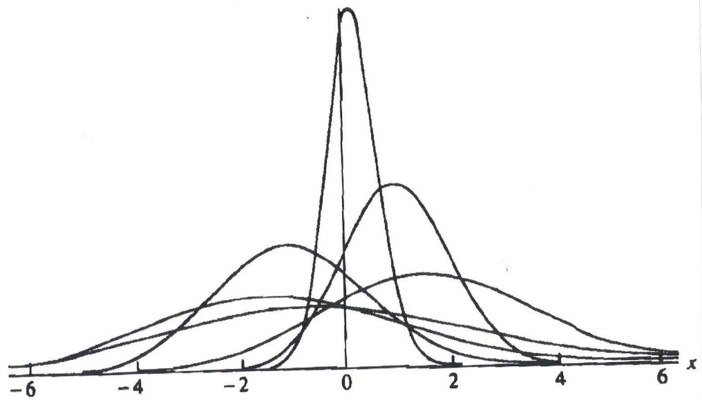
Figure 3.5.4. Members of the same location-scale family
