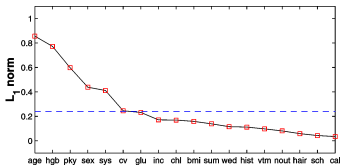
Figure 10. L_1 Norm Scores for the BDES Main-Effects Model.
