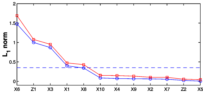
Figure 7. L_1 Norm Scores for the Main-Effects Model Incorporating Categorical Variables ( \circ CKL; \square GACV).
