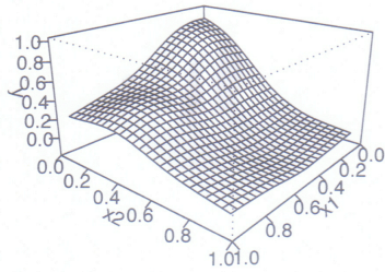
oversmoothed
