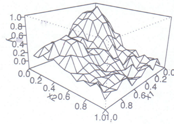
undersmoothed
