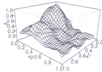
undersmoothed
